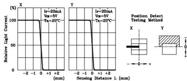
Position Detect Characteristics
